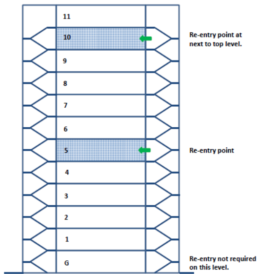
Figure 6.8.3.1 (b). Required re-entry floors when starting at the next to top level.
